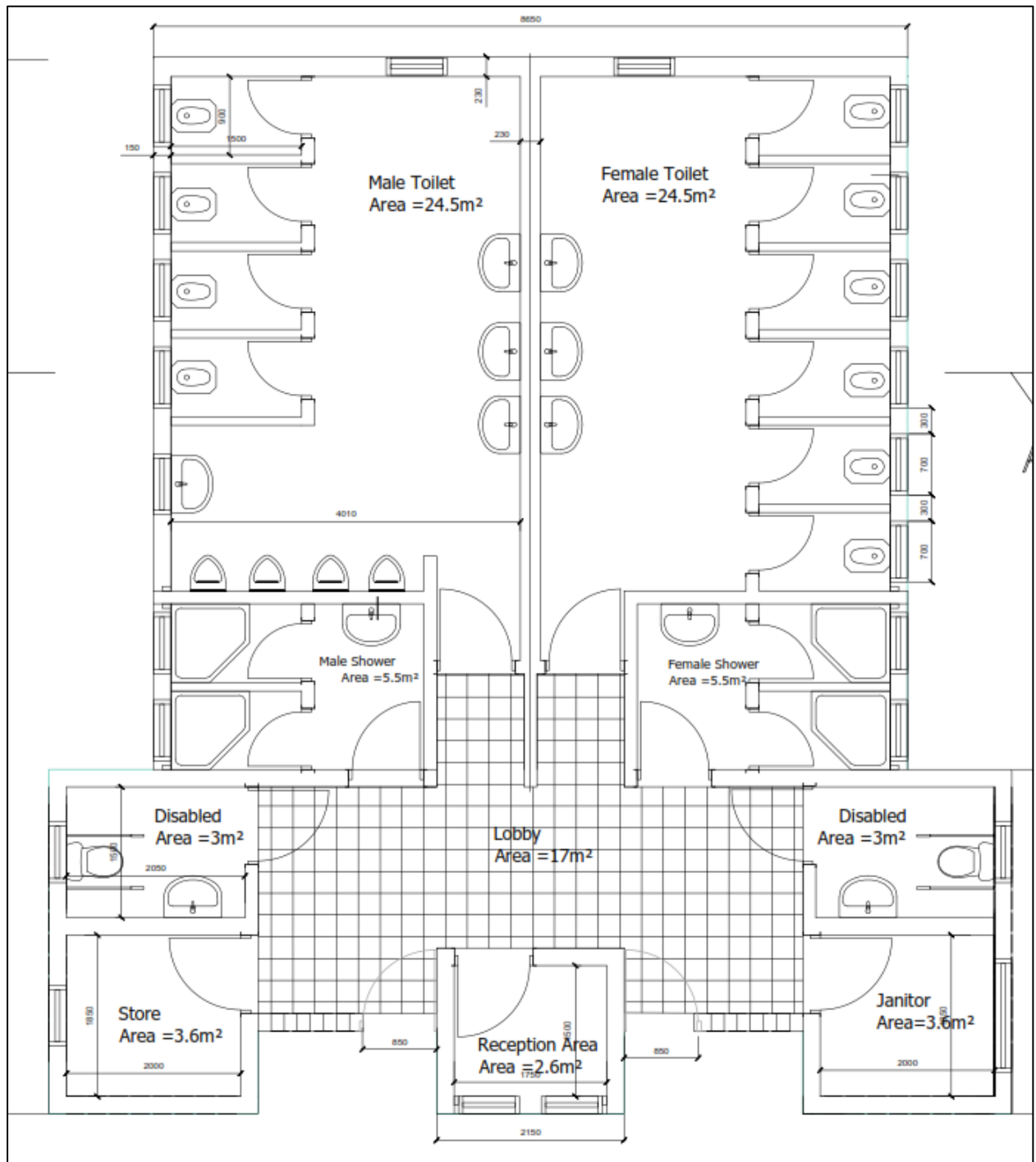
Figure 5: Floor Plan for Public Toilet (Source: Consultant)
